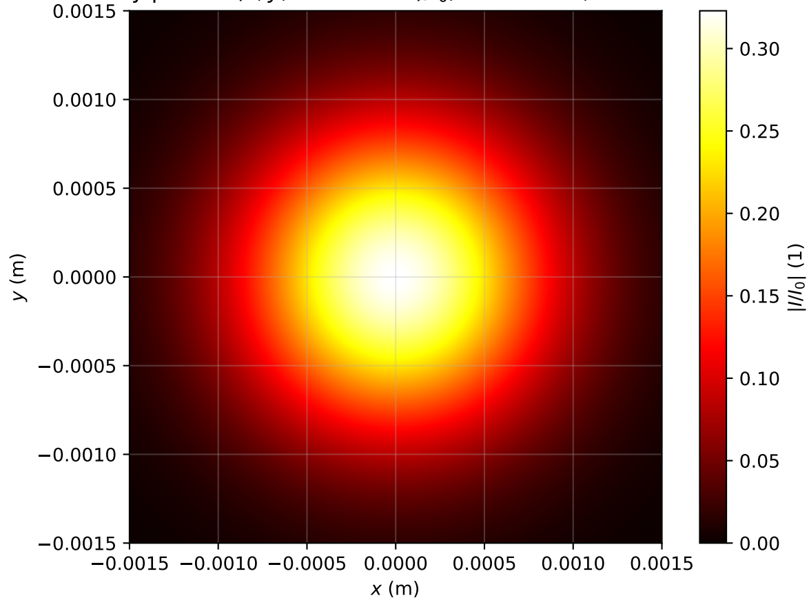
Intensity profile I(x, y, z = 3.344m)/I_0 , P_{in}=0.2P_{cr} , artificial time
